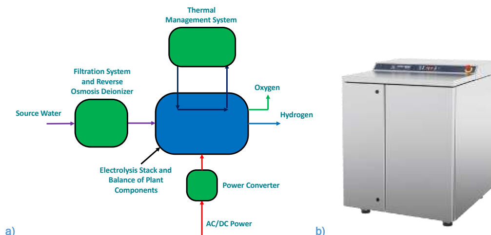
Figure 6. a) Schematic of a typical electrolyzer system, and b) Proton OnSite S Series electrolyzer.
