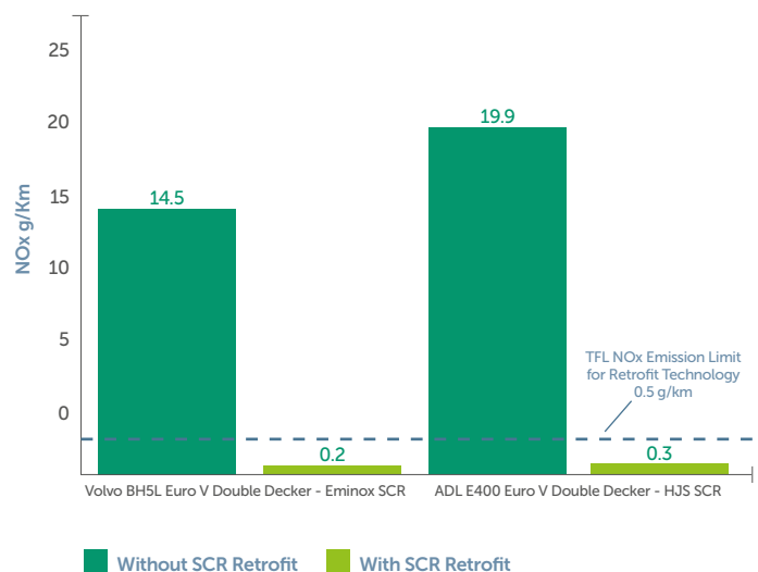
Diagram 3: Vehicle Emissions Testing Results - NO x Emissions for TfL Euro V Buses Before and After SCR Retrofit
